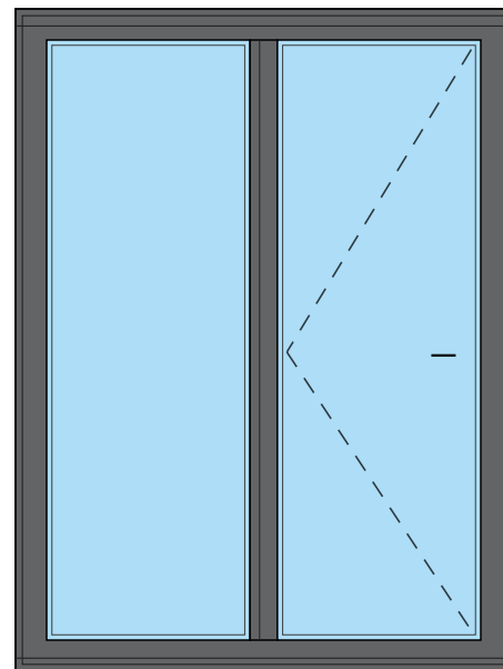
1.5m uPVC Single Door with Side Screen
