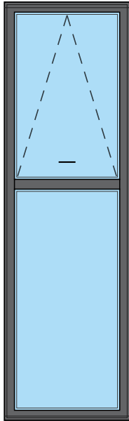
600 x 2000mm uPVC Window with Top Opener
