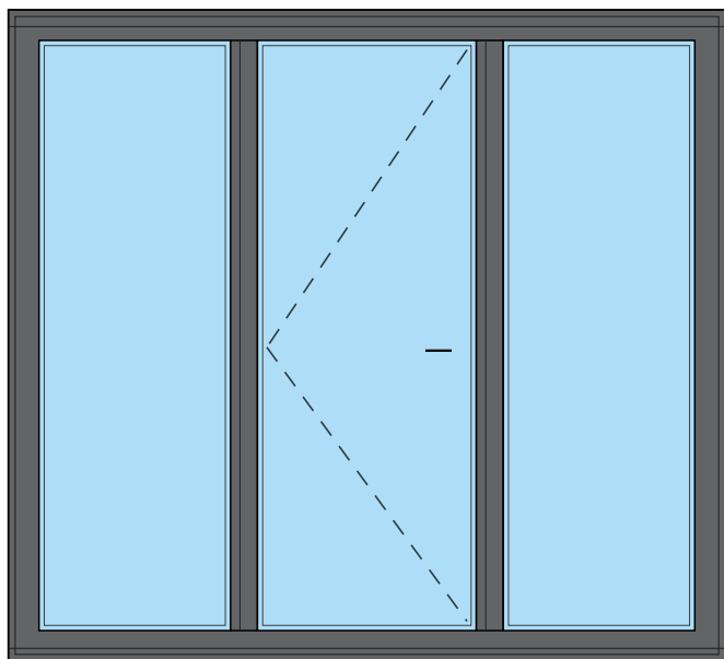
2.2m uPVC Single Door with 2 Side Screens
