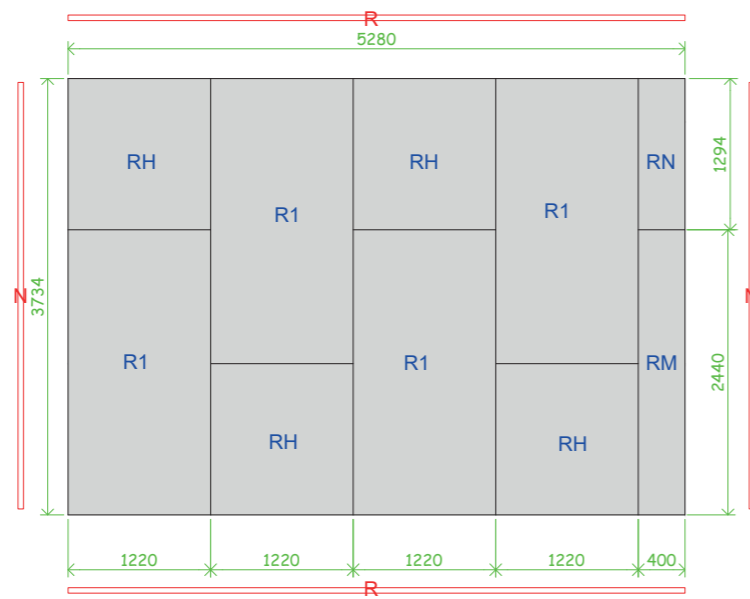
ROOF PANEL PLAN
