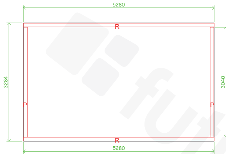
WALL PLATE PLAN
