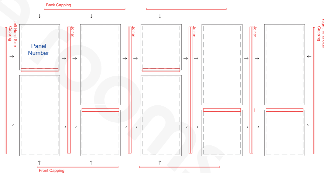
GENERIC FLOOR AND ROOF ASSEMBLY SEQUENCE Note: number of panels will change depending on room dimension
