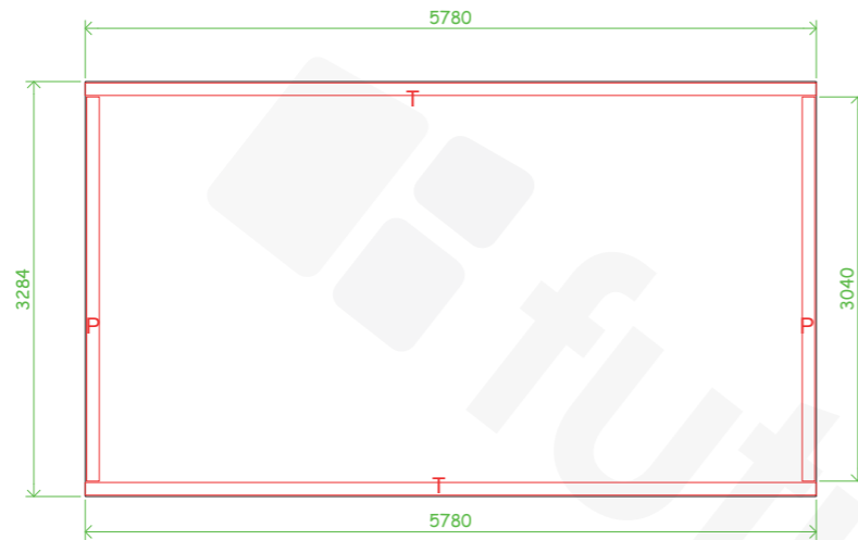
WALL PLATE PLAN
