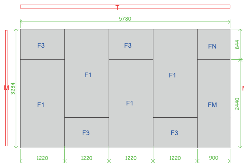
FLOOR PANEL PLAN
