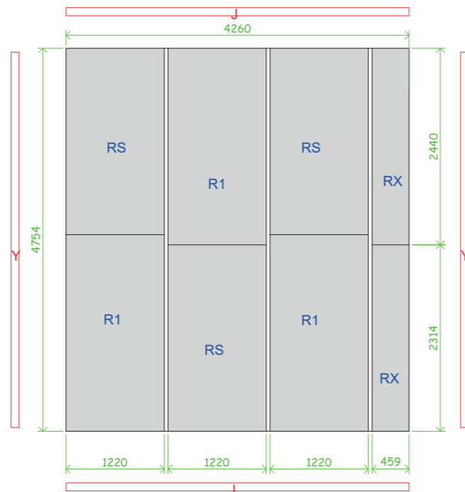
ROOF PANEL PLAN
