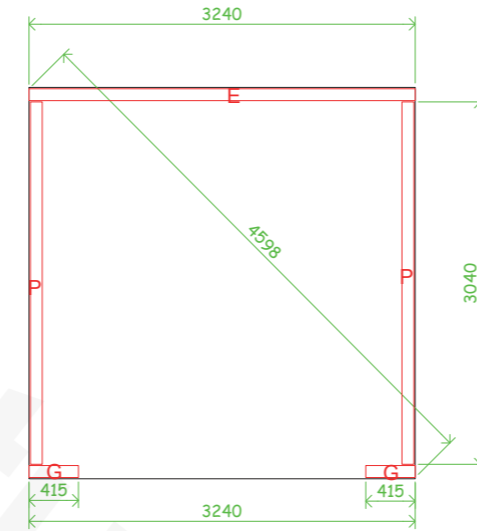
SOLE PLATE PLAN
