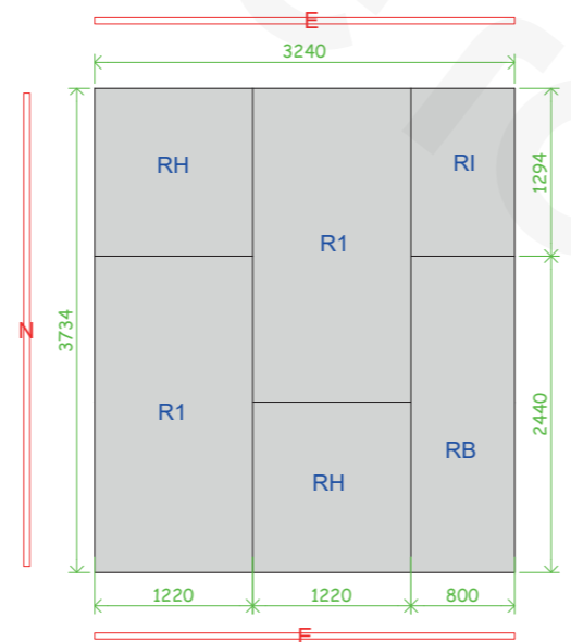
ROOF PANEL PLAN
