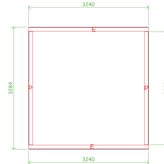
WALL PLATE PLAN
