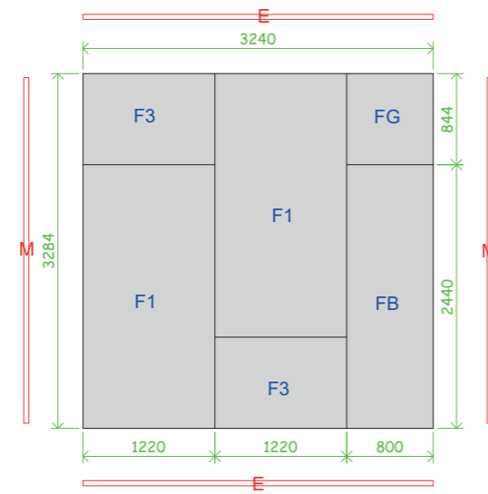
FLOOR PANEL PLAN
